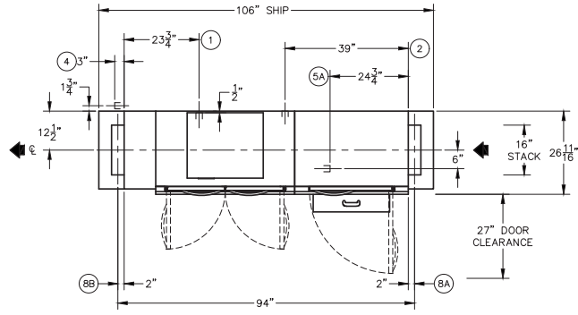
Plan View: Right to Left Model
