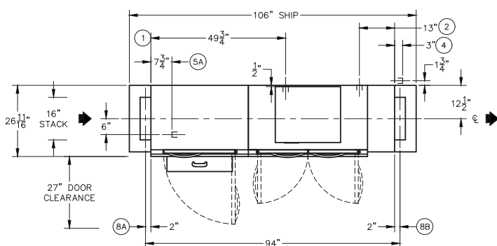
Plan View: Left to Right Model
