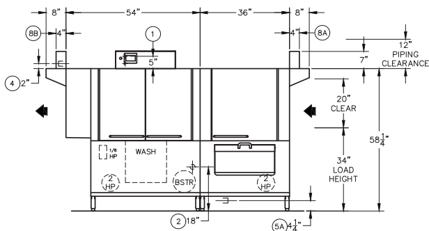
Front View: Right to Left Model
