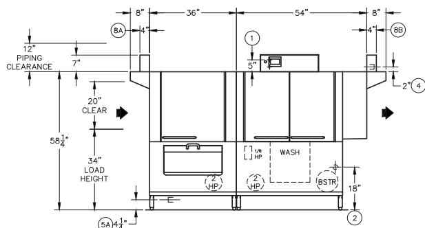
Front View: Left to Right Model
